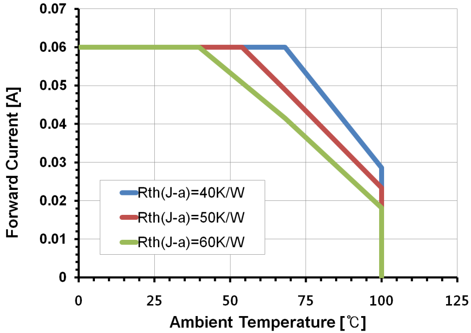
Fig 9. Ambient Temperature vs. Maximum Forward Current, T_{j,max}=125^{\circ}\text{C}
