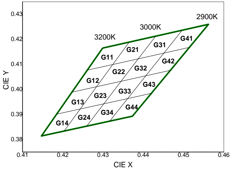
CIE Chromaticity Diagram (Warm white), T_a=25^\circ\text{C} , I_F=40\text{mA}
